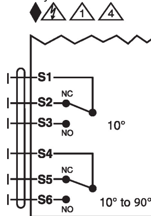
Auxiliary Switches
