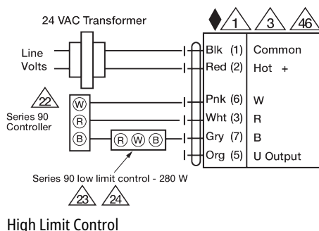
High Limit Control
