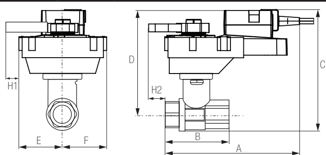
Dimensions (Inches [mm])
