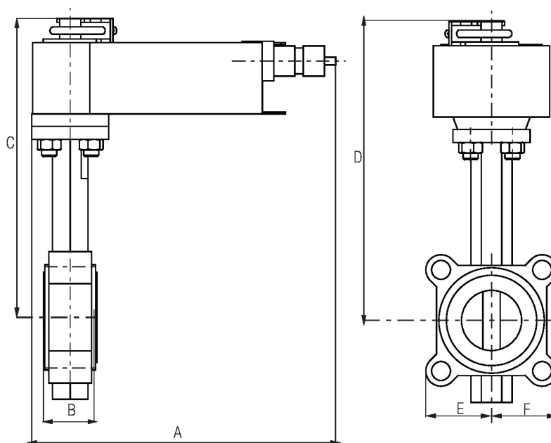
Valve with AFR Actuator
