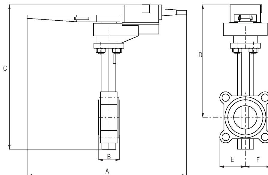
Valve with ARB/GRB Actuator
