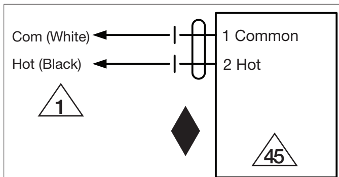
24 VAC/DC
