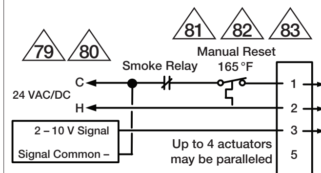
Parallel wiring
