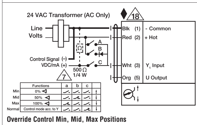
Override Control Min, Mid, Max Positions
