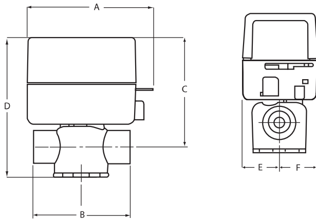
Dimensions (Inches[mm])
