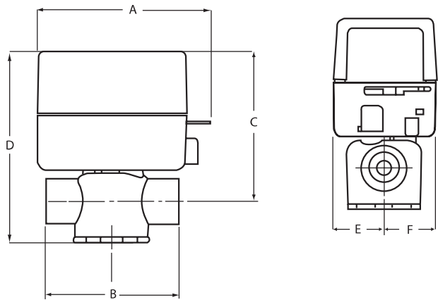
Dimensions (Inches[mm])
