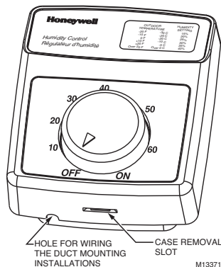
Fig. 2. H8908B,C control.
