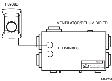
Fig. 19. Typical wiring diagram for HR150, HR200, ER150 and ER200 Ventilator or DH90 Dehumidifier applications.
