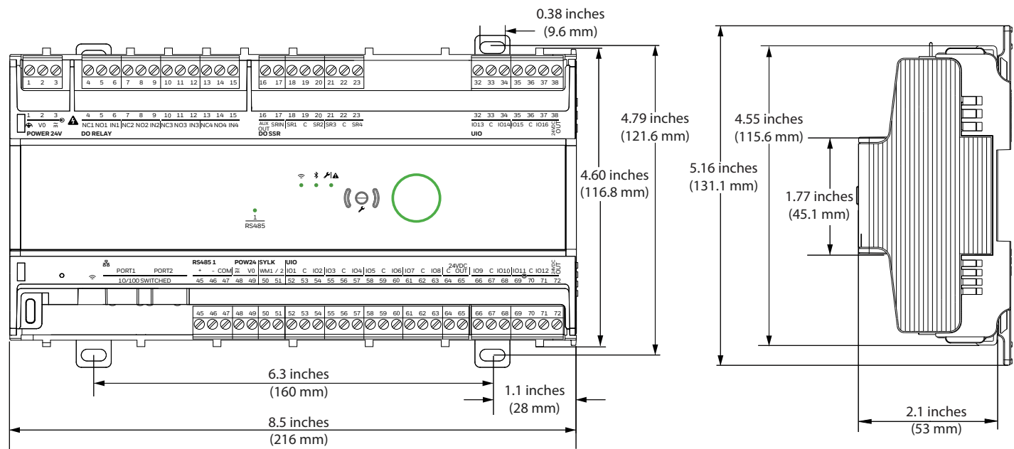
Fig. 2 Unitary controller large dimensions
