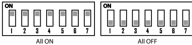
Fig. 25 MS/TP MAC Address Details
