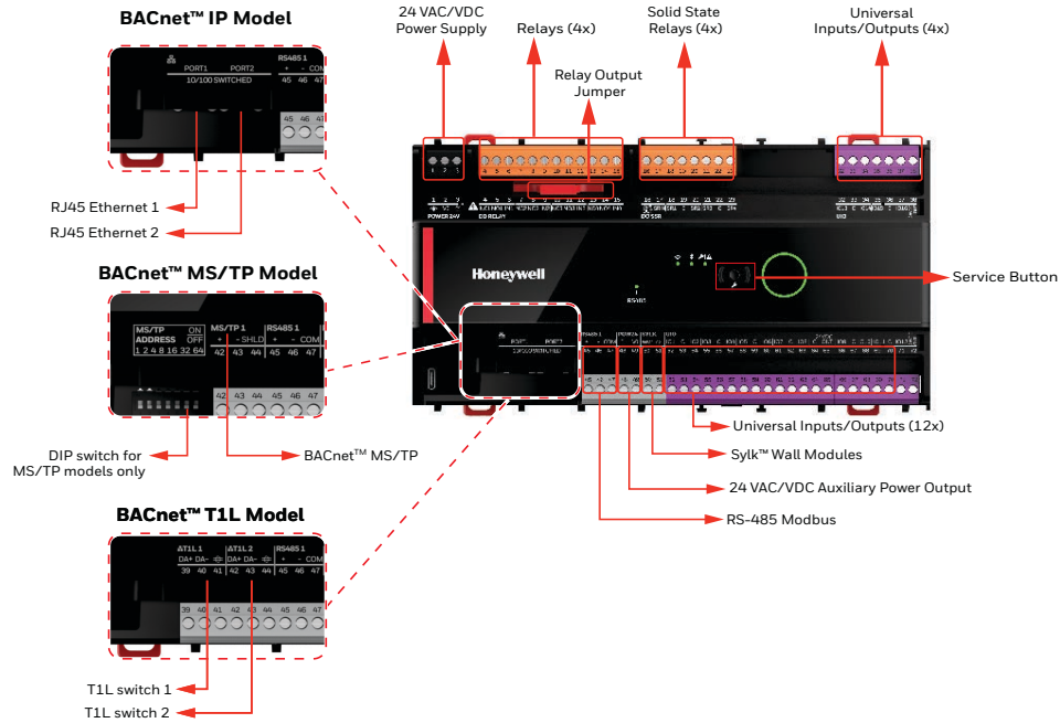
Fig. 4 Hardware Overview
