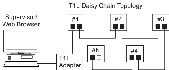
Fig. 27 T1L Daisy chain Topology
