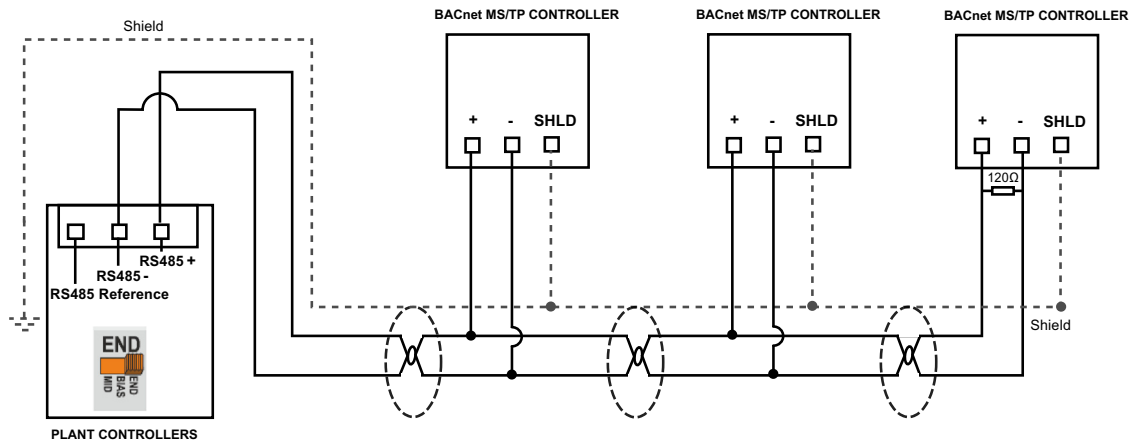
Fig. 22 Connection to a BACnet™ MS/TP Bus
