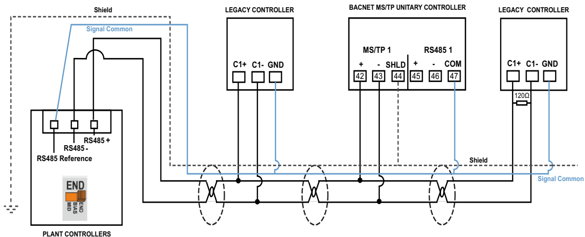
Fig. 23 Connection to BACnet MS/TP Bus (signal common)
