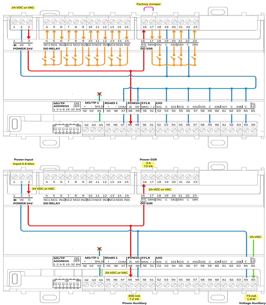
Fig. 15 Internal Wiring Small controller
