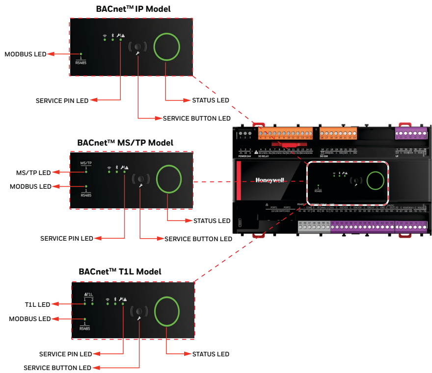
Fig. 32 LED Interface
