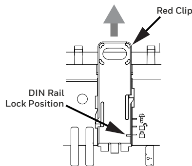
Fig. 7 Lock Position
