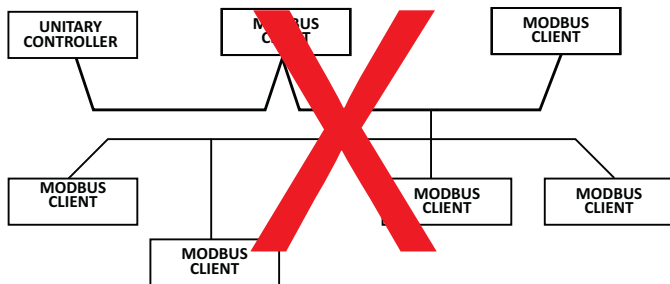
Fig. 30 Prohibited Wiring Topology (example)
