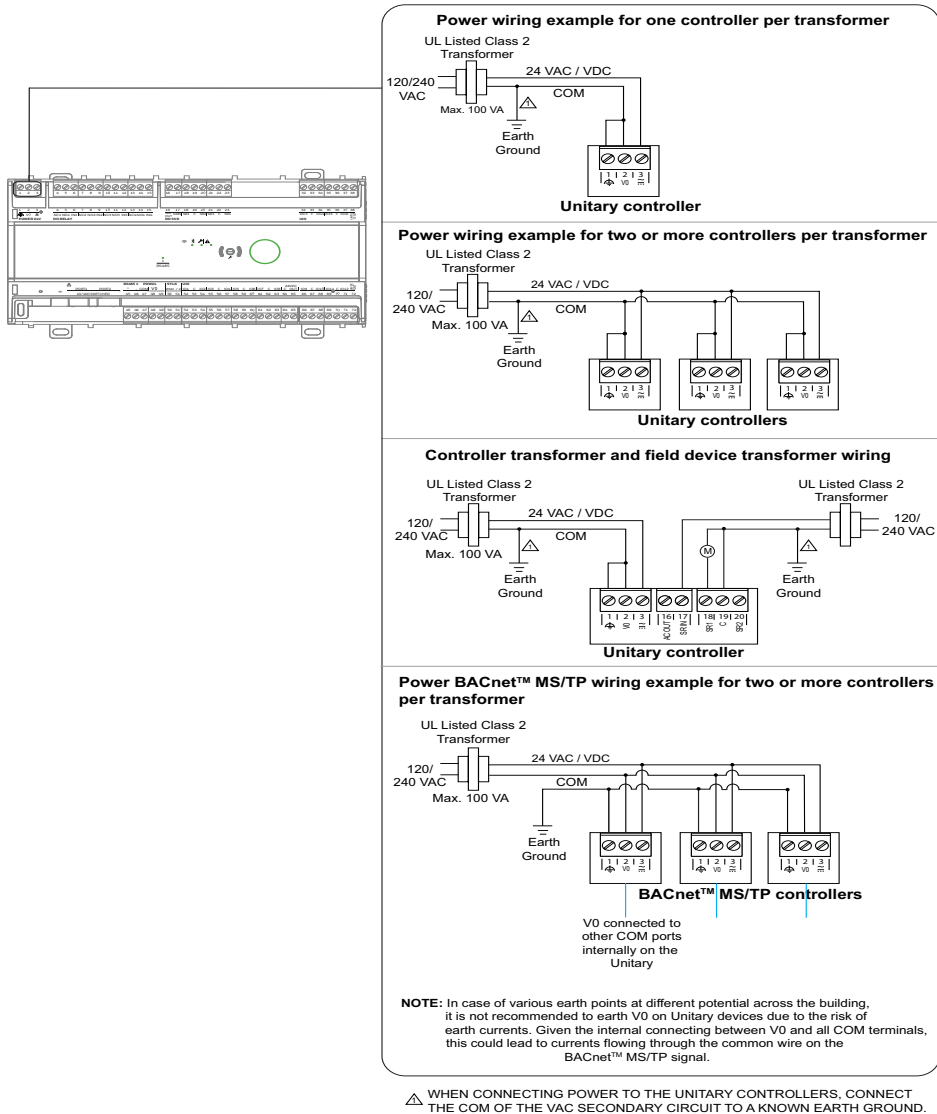
Fig. 12 Power Wiring Examples
