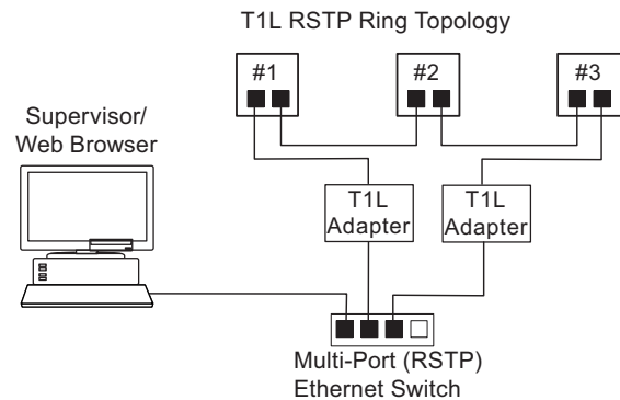
Fig. 28 T1L Ring Topology
