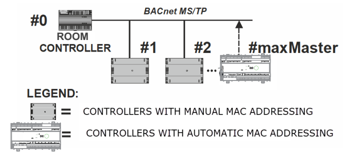
Fig. 24 Automatic MAC Addressing
