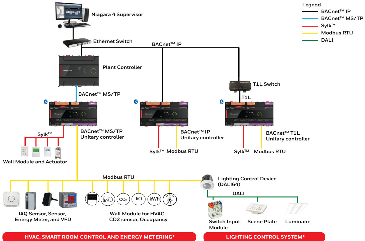
Fig. 5 System Overview
