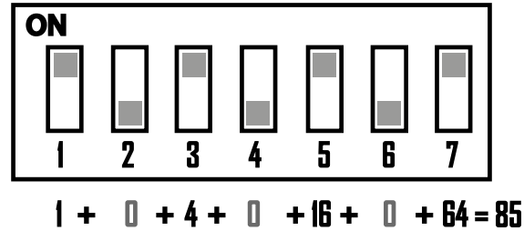
Fig. 26 Calculating the MAC Address
