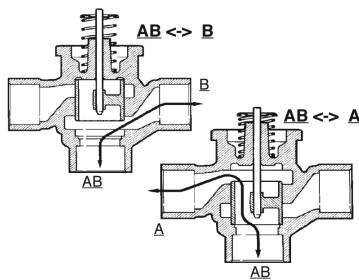
Fig. 2. Fluid flow of 3-way valves
