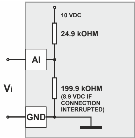
Fig. 31. Analog input impedance setpoint (input circuit for NTC10k \Omega , NTC20k \Omega , wall module setpoint)
