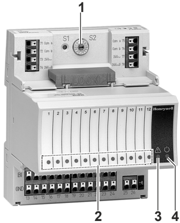
Fig. 15. XF823 Panel Bus BI Module (shown with XS823 terminal socket)
