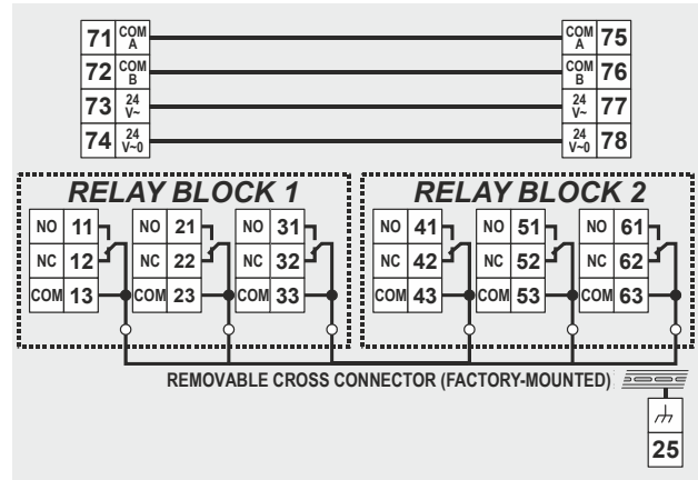
Fig. 20. Terminal assignment and internal connections
