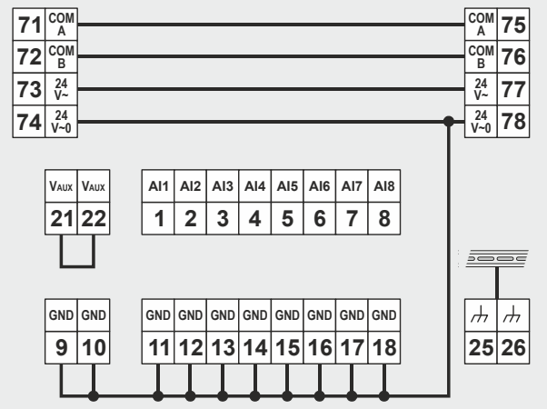
Fig. 7. Terminal assignment and internal connections
