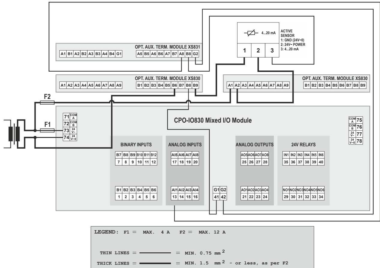
Fig. 34. CPO-IO830 Connection example (for current inputs)
