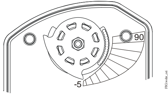
Figure 6: Washer Orientation on Actuator
