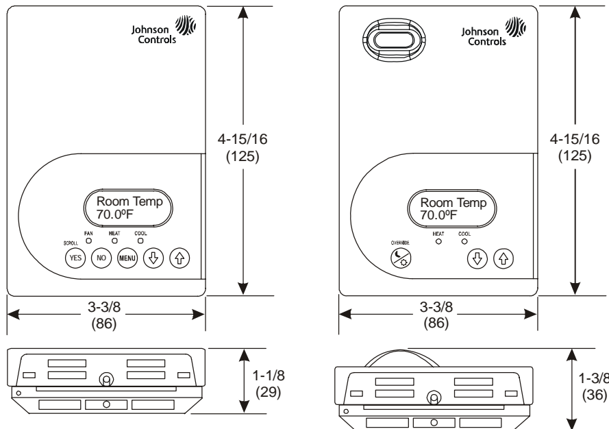
TEC264Z-2 Rooftop Controller (Left) and TEC2647Z-2+PIR Zone Controller (Right) Dimensions, in. (mm)
