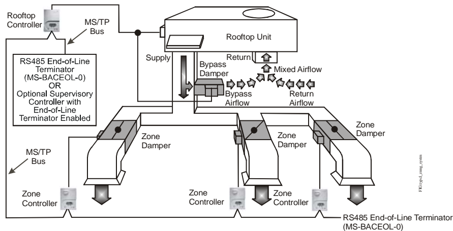
Typical Zoning Control System Installed on a Single MS/TP Bus
