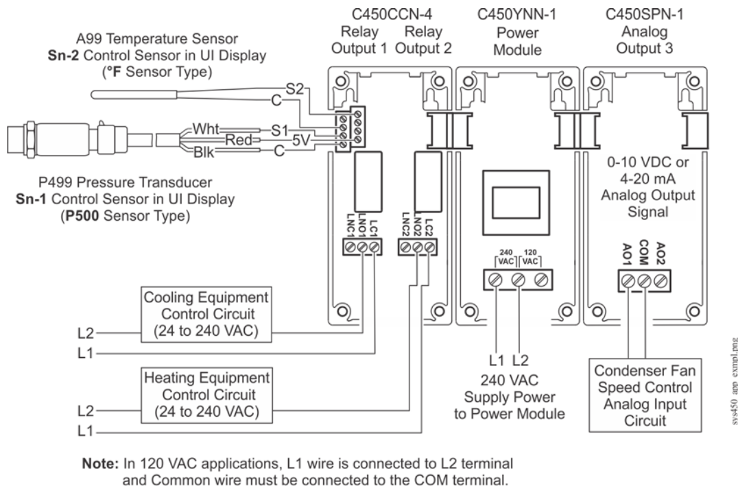
Figure 3: System 450 Heat/Cool System with Condenser Fan Speed Control Example
