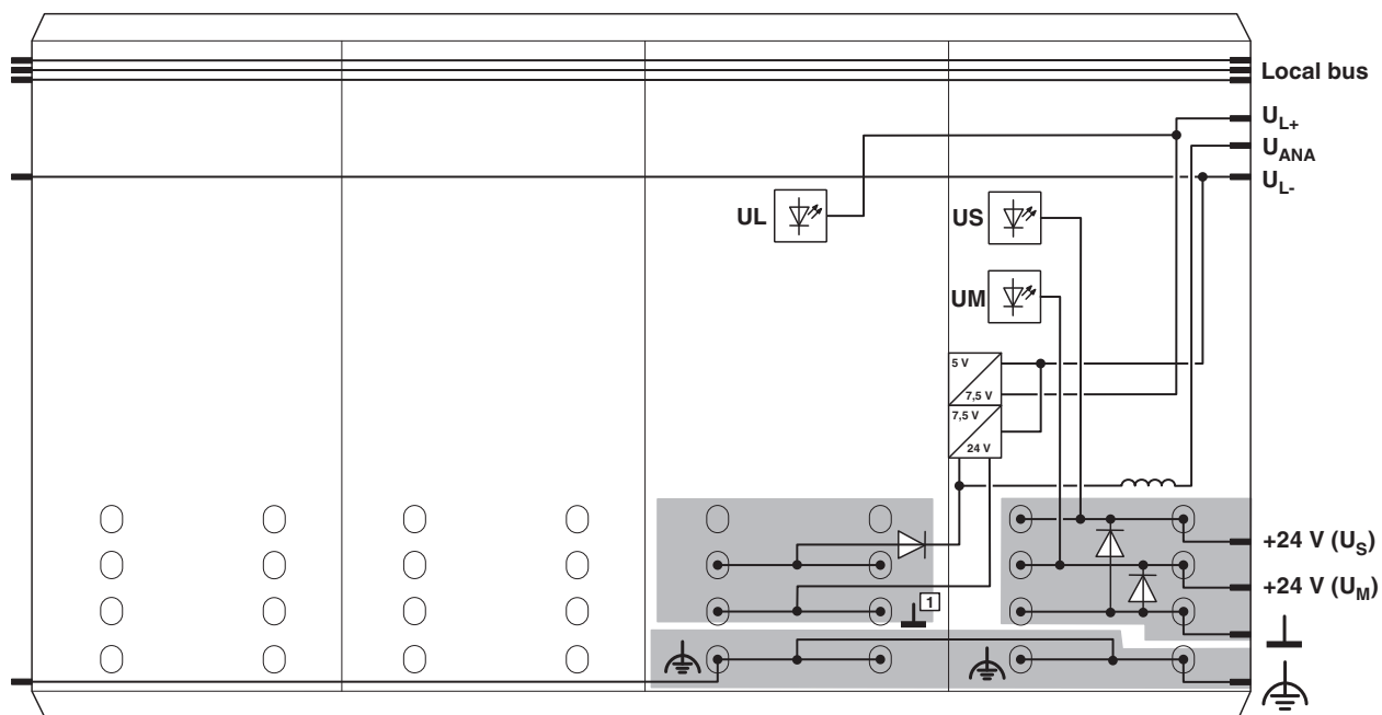
Figure 1 Internal wiring of the terminal points
