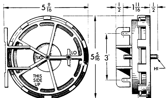
Figure-2 Dimensions.
