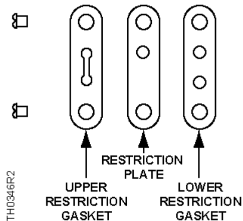
Figure 1. Restriction Plate Kit Assembly.
