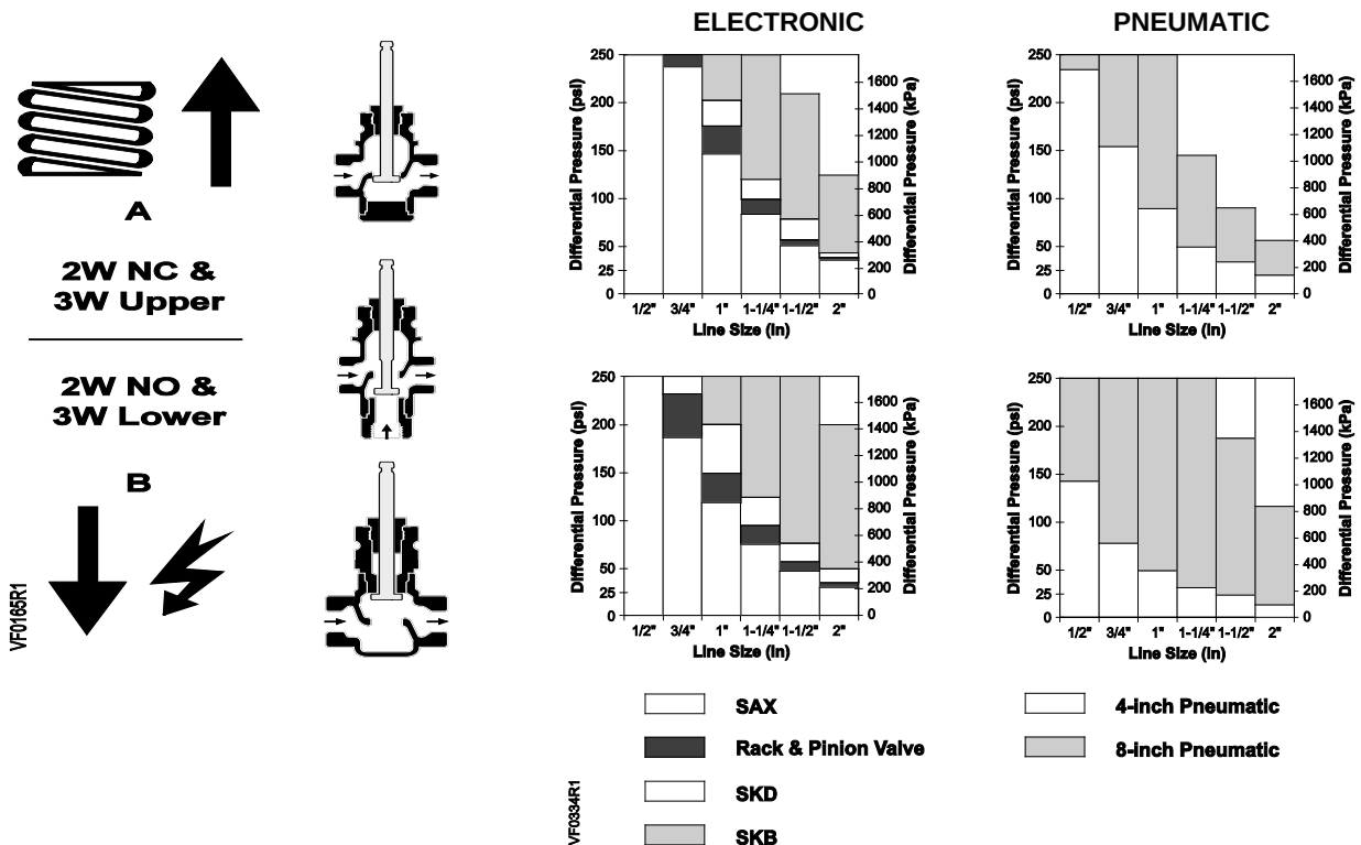
Figure 2. Close-off Pressures.
