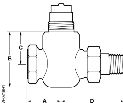
Female NPT x Union Male FxUM
