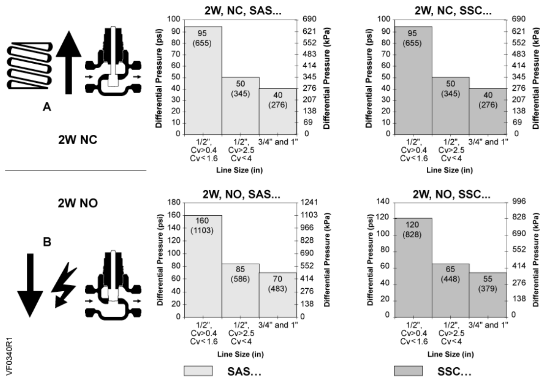
Figure 2. Close-off Pressures.
