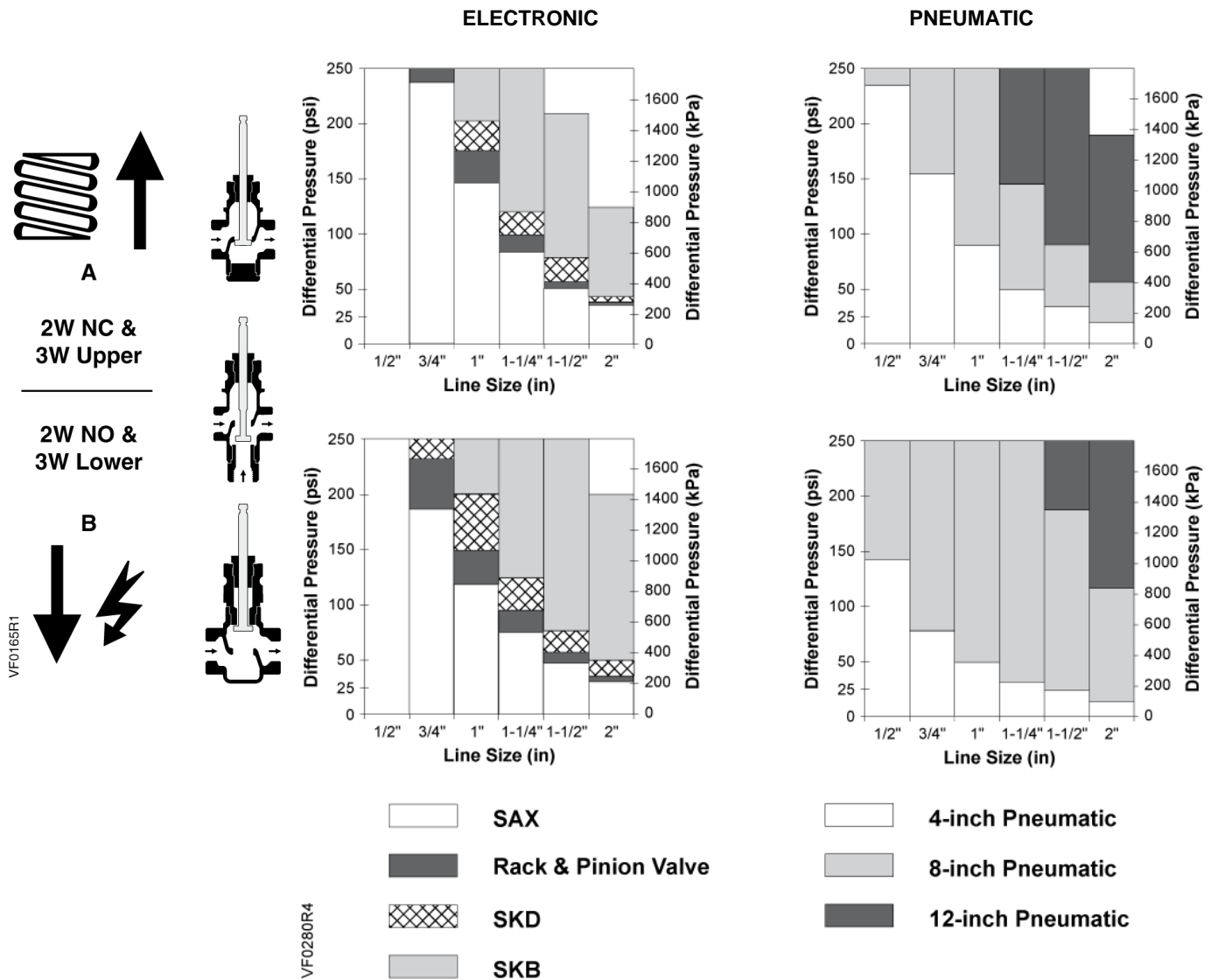
Figure 4. Close-off Pressures.
