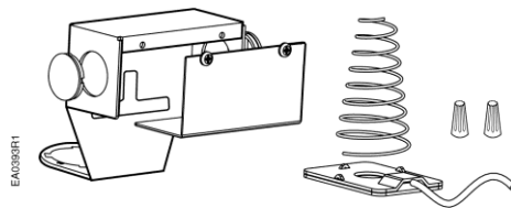
Figure 1. Packing Heating Element For Use with SKD Actuators.
