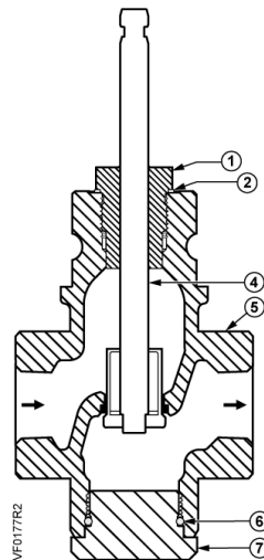
Figure 8. Normally Closed Valves 1/2-inch to 2-inch (15 to 50 mm) Valve Size.
