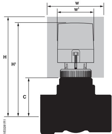
Thermic Actuator: 2-Way Valve Assembly Service Envelope
