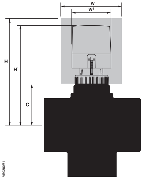
Thermic Actuator: 3-Way Valve Assembly Service Envelope
