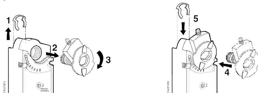
Figure 10. Mechanical Range Adjustment.
