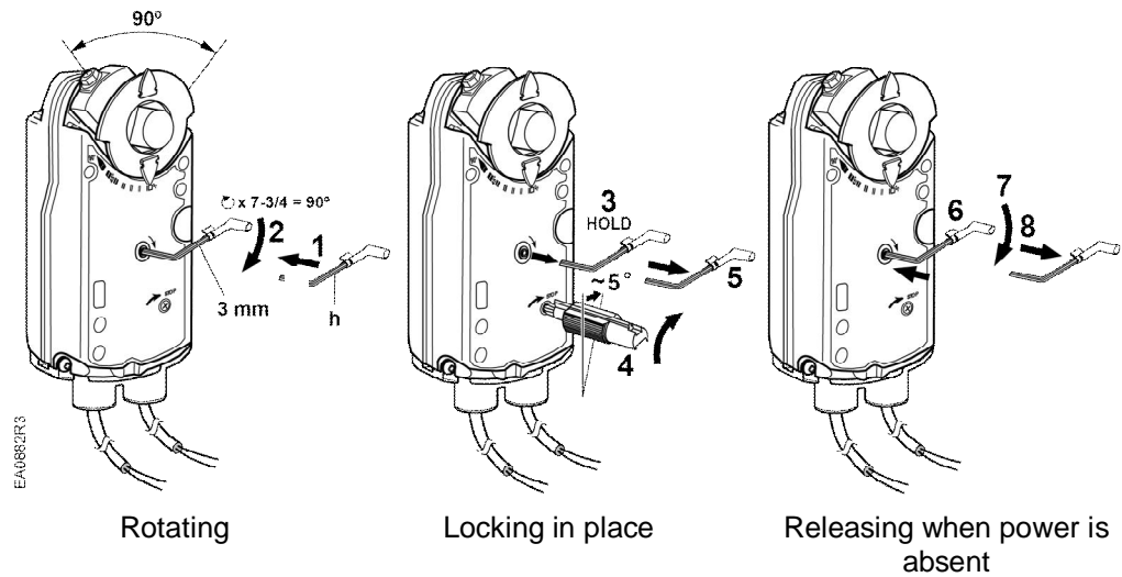
Figure 9. Manual Override.
