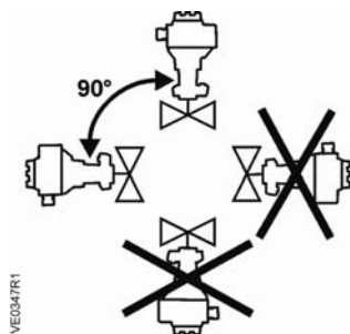
Figure 1. Acceptable Outdoor Mounting Positions with Weather Shield.
